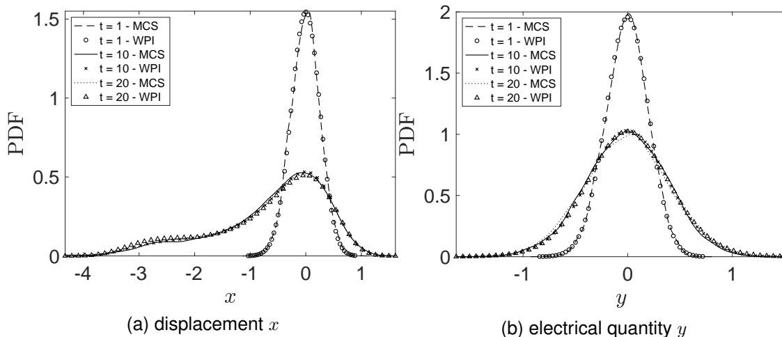
Fig. 3: Marginal response PDFs of a nonlinear energy harvester with \zeta = 0.1 , \kappa = 0.65 , \alpha = 0.8 , \delta = 0.2 , S_0 = 0.05 and fractional derivative order r = 0.75 for three (non dimensional) time instants t = 1 , t = 10 and t = 20 . Comparison with MCS data (10, 000 realizations).
