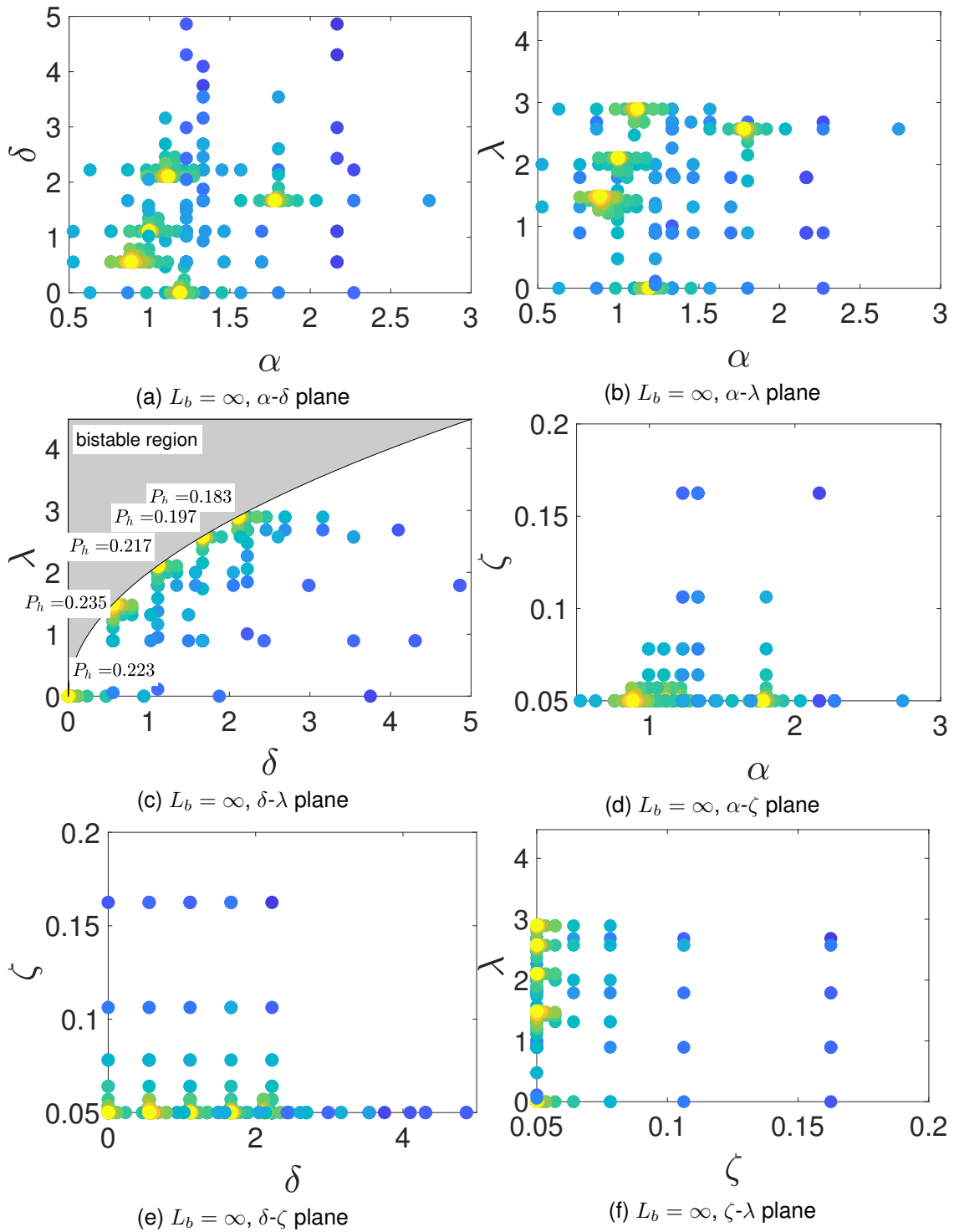
Fig. 5: 2D projections of computed points (color varies with iteration count). Optimization by GPS algorithm with z = [\alpha, \delta, \zeta, \lambda]^T \in [0.5, 3] \times [0, 5] \times [0.05, 0.2] \times [0, 2\sqrt{\delta}] , \kappa = 0.65 , r = 1 and unconstrained probability of failure ( L_b = \infty ).
