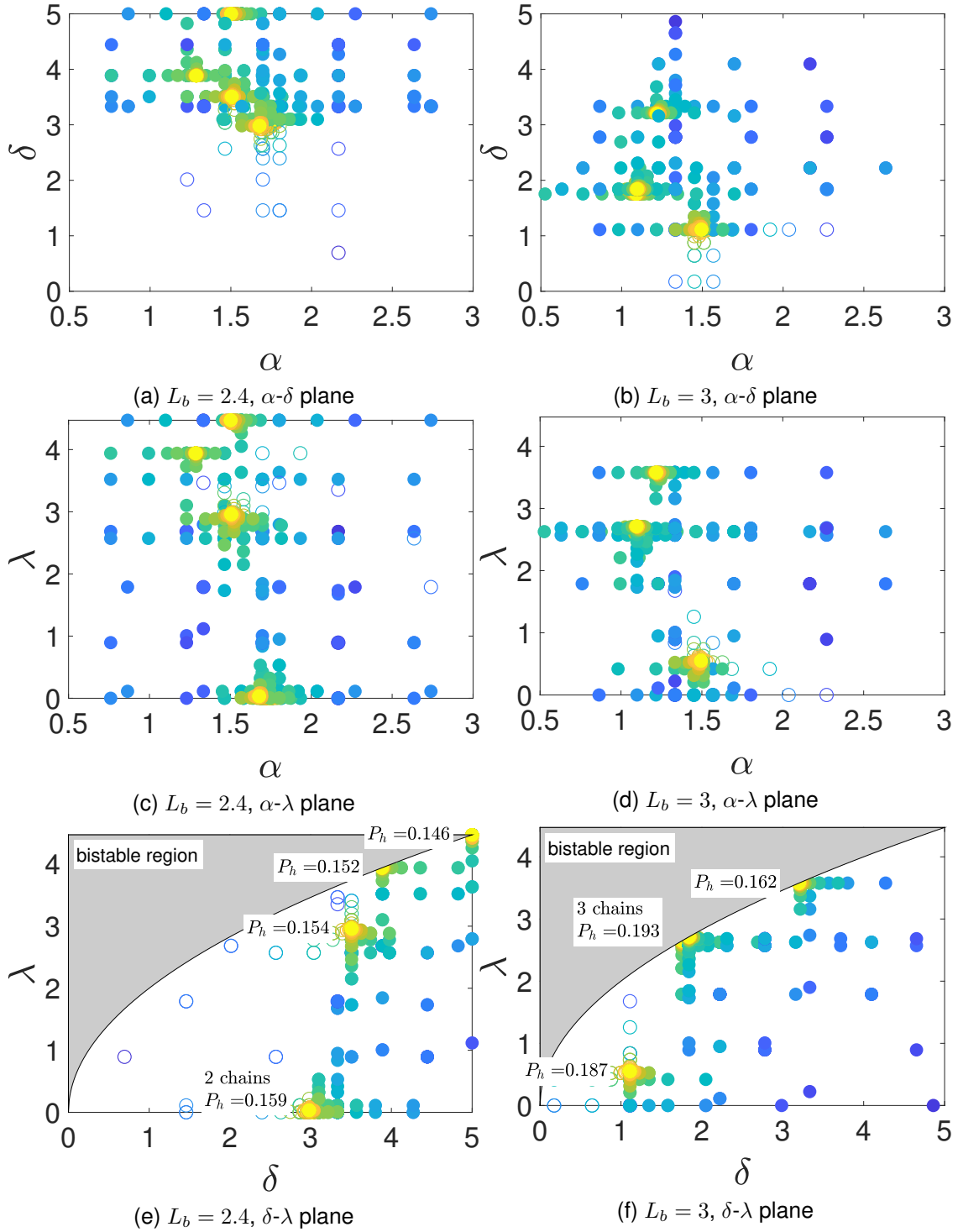
Fig. 6: 2D projections of computed points (color varies with iteration count and unfilled circles correspond to probabilities of failure larger that \epsilon ). Optimization by GPS algorithm with z = [\alpha, \delta, \zeta, \lambda]^T \in [0.5, 3] \times [0, 5] \times [0.05, 0.2] \times [0, 2\sqrt{\delta}] , \kappa = 0.65 , r = 1 and constrained probability of failure with L_b equal to 2.4 (6a,6c,6e) and 3 (6b,6d,6f) and \epsilon = 10^{-3} .
