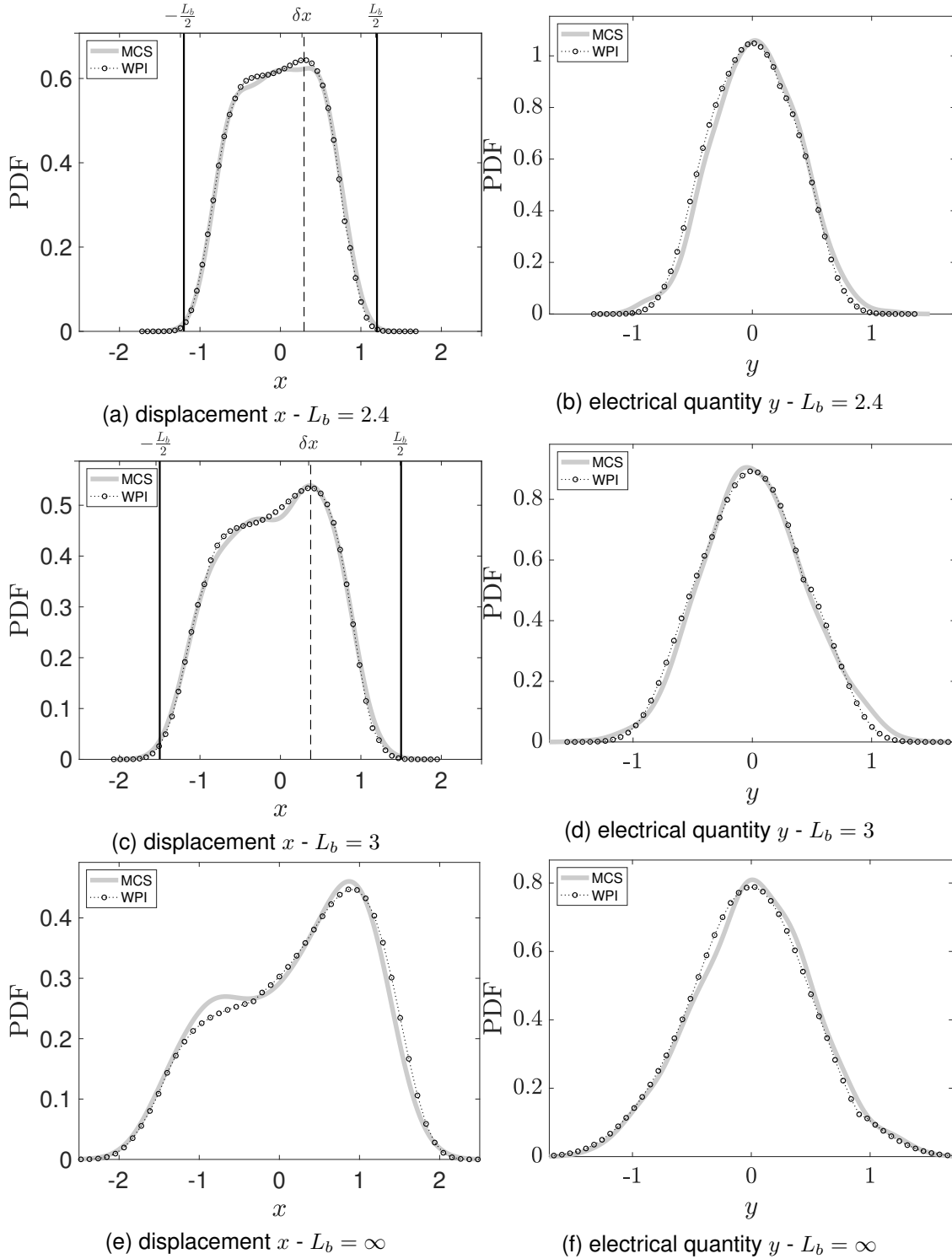
Fig. 8: Response PDFs of three optimal designs corresponding to box size parameter L_b values of 2.4, 3 and \infty ; see second, eighth and ninth rows of Tab. 3, respectively, for optimal design parameters (\alpha^*, \delta^*) , shift parameter \delta x , mean harvested power P_h and probability of failure P_f .
