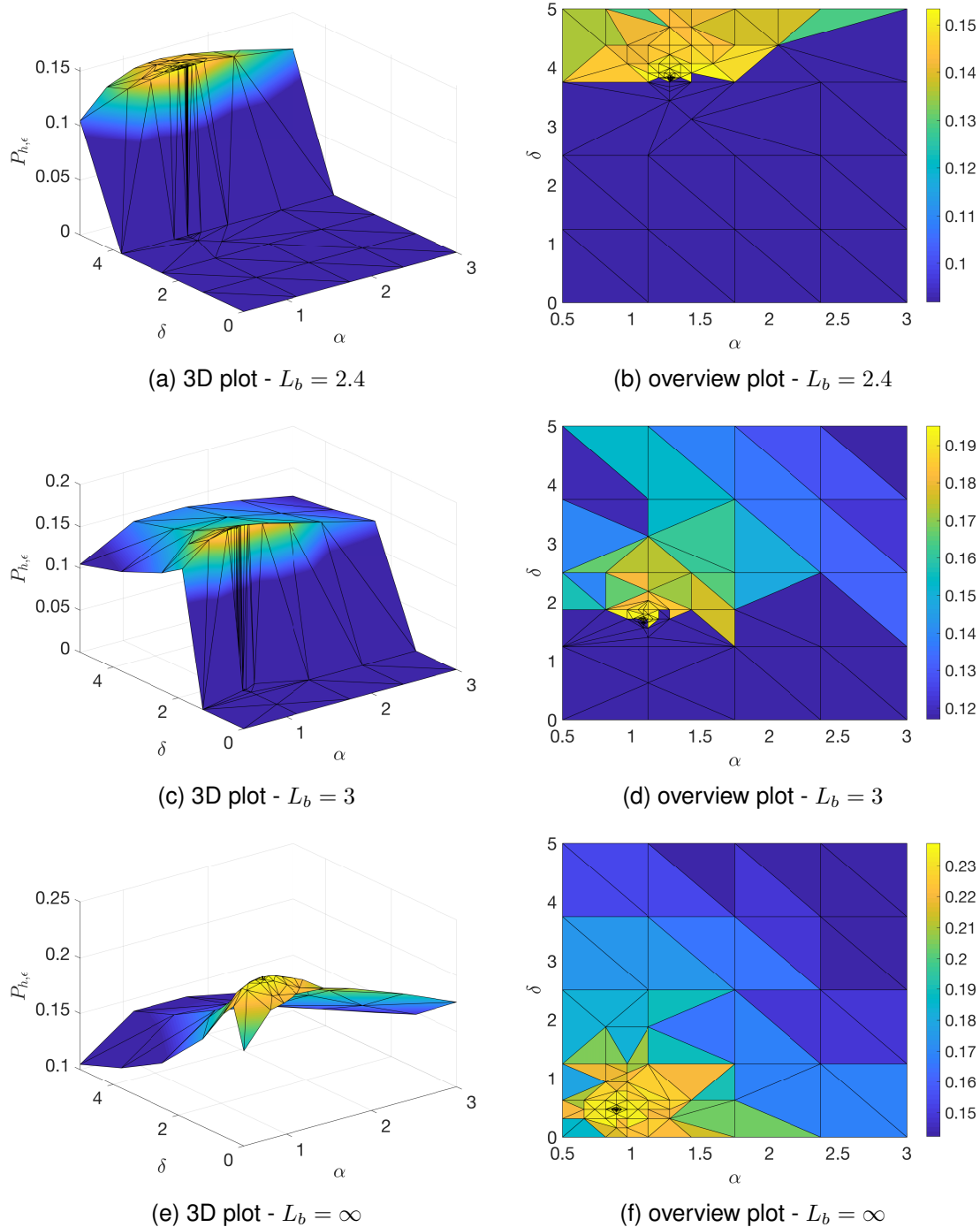
Fig. 7: Stationary mean harvested power P_h . Optimization by GPS algorithm with z = [\alpha, \delta]^T \in [0.5, 3] \times [0, 5] , \lambda = 2\sqrt{\delta} , \zeta = 0.05 , \kappa = 0.65 , r = 1 . (a),(c) and (e): 3D surface plots with gradient coloring. (b),(d) and (f): overview plots with flat coloring.
