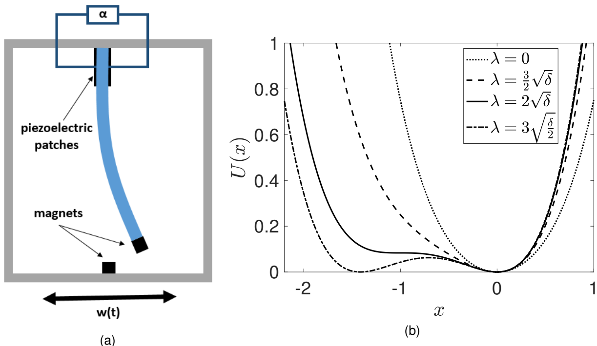
Fig. 1: (a) Schematic representation of the electromechanical energy harvesting device. (b) Various shapes of the potential function for \delta = 1 .
